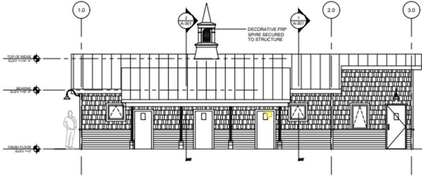
2 SOUTH ELEVATION A-001 SCALE: 1/4" = 1'
