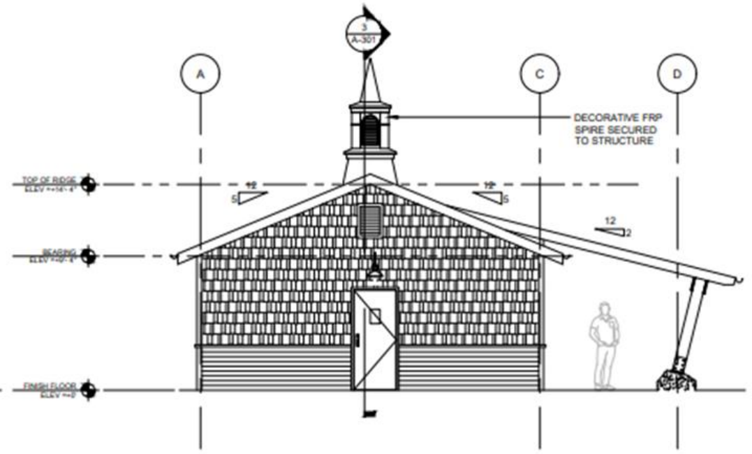
1 WEST ELEVATION A-001 SCALE: 1/4" = 1'
